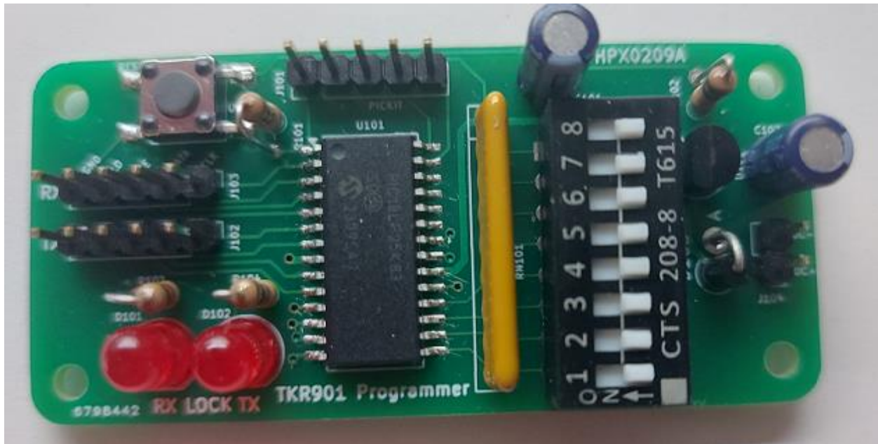
Figure 1 TKR901 Programming Module
